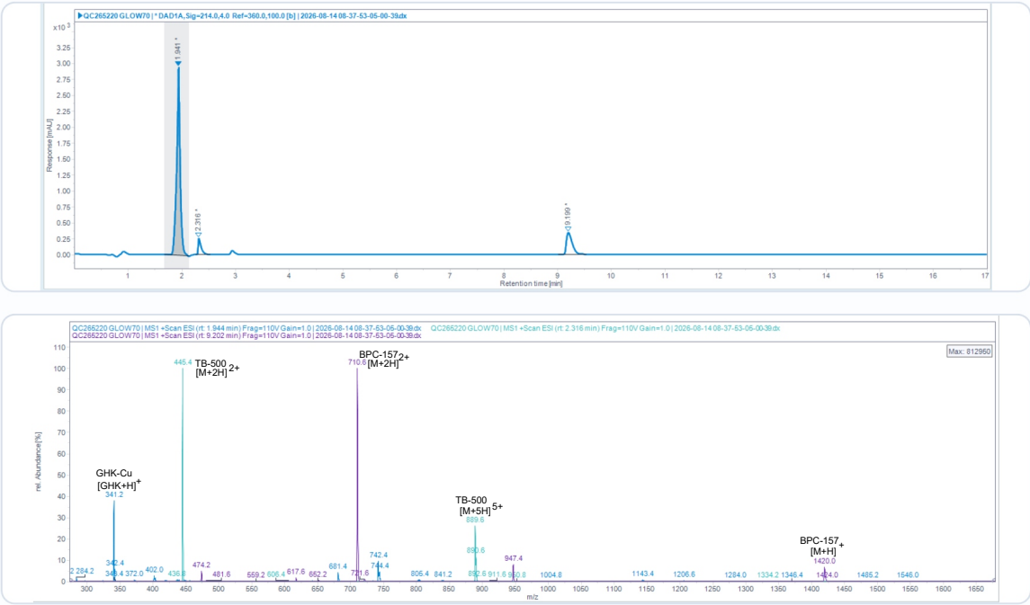
HPLC Chromatogram · Retention Time 1.941, 2.316, 9.199 min
